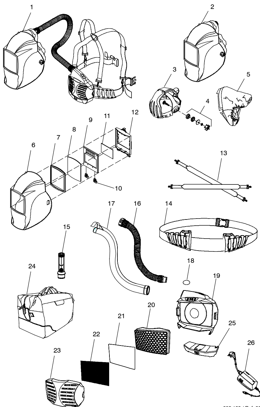
Figure 4-1. AirArmor – Powered Air Purifying Respirator (PAPR)
